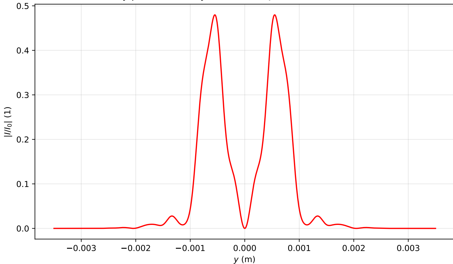
Intensity profile I(x=0, y, z=1.513)/I_0 , P_{in}=6.0P_{cr} , artificial time
